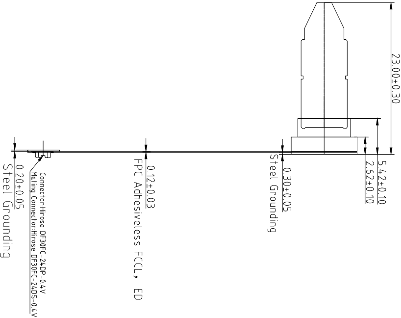
SIDE VIEW
